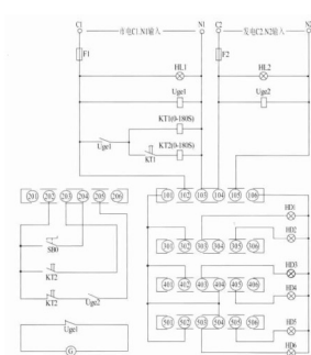
CHCH40-1000-3200A带发电机接线
