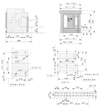
图7-7 HCW1-6300(In=6300A)抽屉式(三级)
