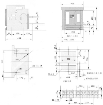
图7-7 HCW1-6300(In=6300A)抽屉式(三级)
